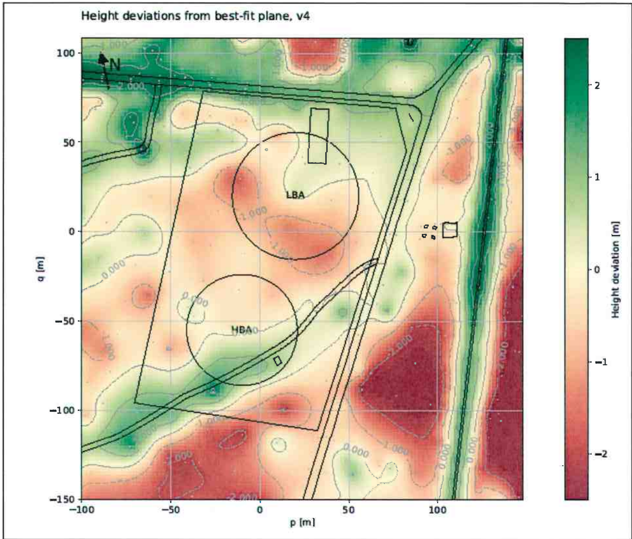
Figure 2-3: example of LOFAR configuration in scale include current height profile
